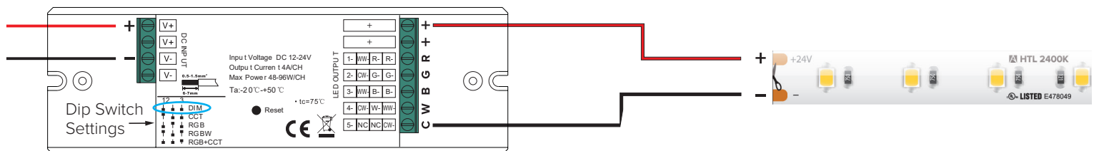
FIGURE 2 - Single Color (2-Wire) Wiring Diagram
