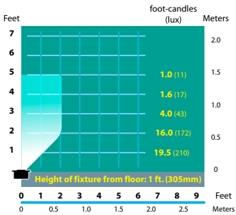
SL-02-3L Half Spread Photometrics
