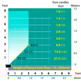
SL-02-AL Half Spread Photometrics
