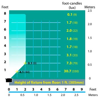
SL-02 Half Spread Photometrics
