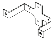
Mounting Bracket 7MBC964501 Qty: 1pc
